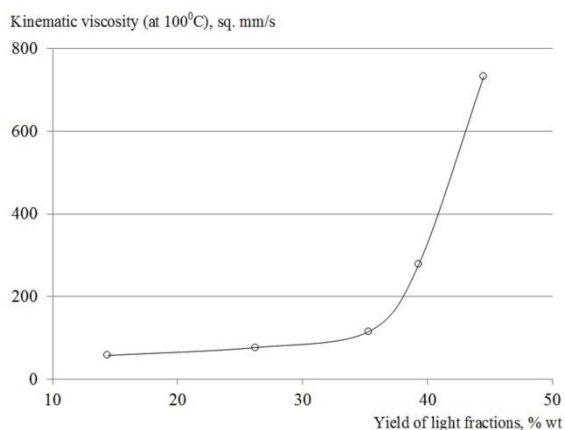
Figure 3. Dependence of kinematic viscosity (at 100°C) of the heavy residue of thermal cracking on the yield of light fractions at T=450^{\circ}\text{C} and P= 3 \text{ atm}
