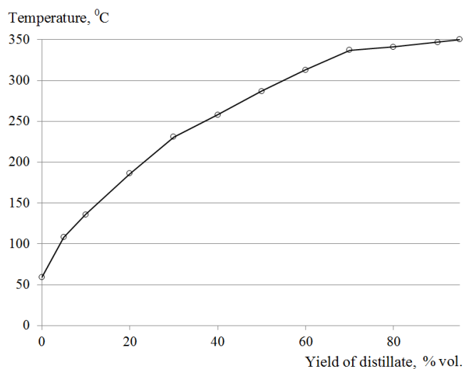
Figure 6. A typical distillation curve of Ryazan fuel oil cracking in the presence of an initiator
