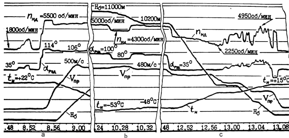
Figure 1. Typical changes in civil aircraft engine modes in flight: a - takeoff taxiing; takeoff; climb; b - en route cruise; c - descent operation, landing approach, landing, reverse thrust.
