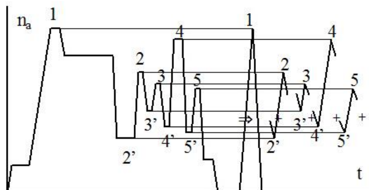
Figure 3. GTE loading cycle counting using the system of simple loading cycles
