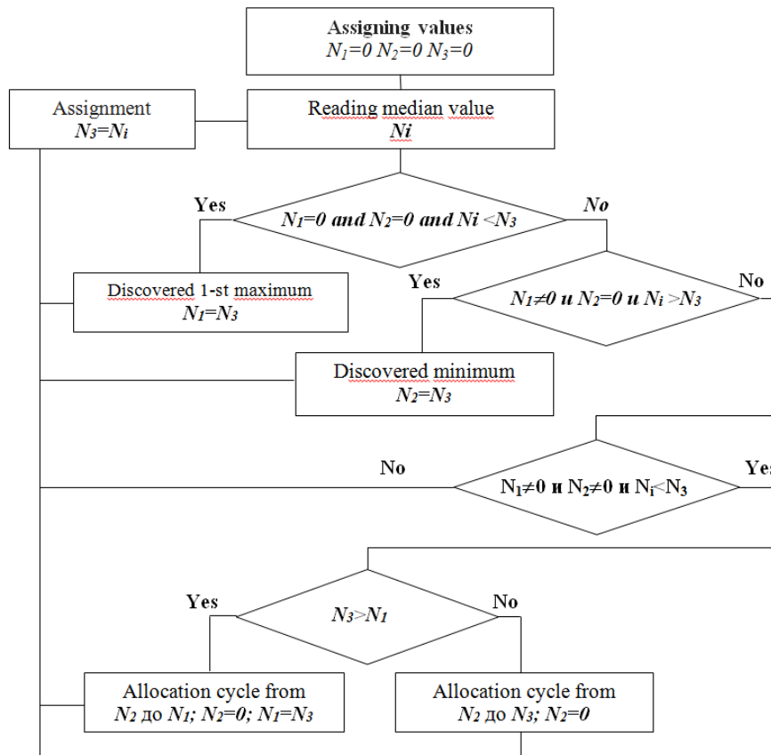
Figure 5. Flowchart of the algorithm for distinguishing “simple” cycles
