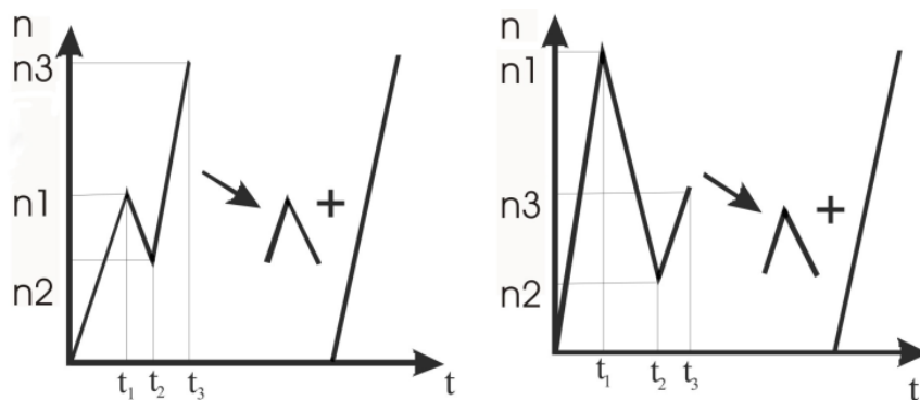
Figure 4. Possible allocation of the main and additional simple loading cycles with regard to the sequence of three extrema
